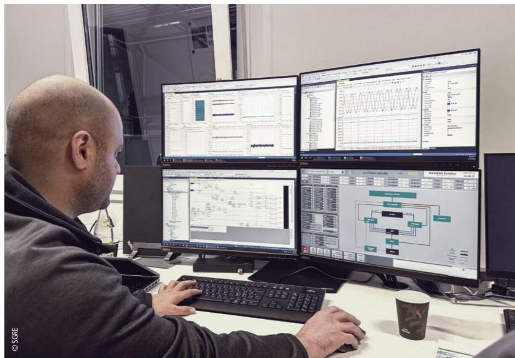
Beckhoff TwinCAT software plays an important role in the SGRE test rig, including TwinCAT 3 Scope View for data analysis (both top screens), TwinCAT 3 Target for Embedded Coder® (bottom left), and TwinCAT 3 HMI for convenient system operation (bottom right).
