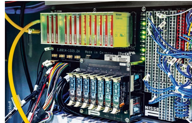
The EtherCAT plug-in modules of the EJ series (above) – mounted on the customer-specific signal distribution board – result in a highly compact, standardized, and yet flexible I/O level.
