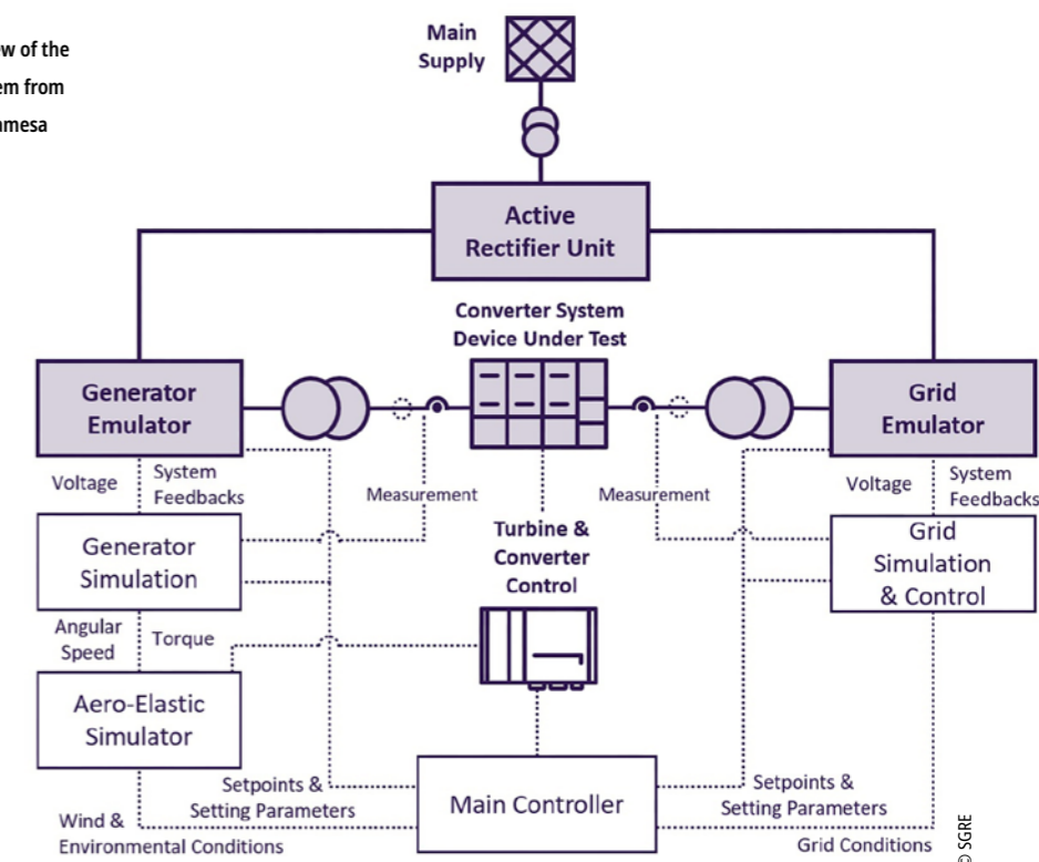
System structure of the Grid-Converter Test Rig
